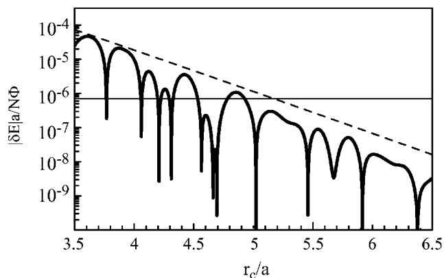
FIG. 4. Determination of r_c for \lambda=3 . The heavy curve is our estimate of \delta E(r_c) obtained from simulations at \tilde{T}=8.84 \times 10^{-3} , with r_l=10a . The dashed line is the analytic upper bound on \delta E(r_c) from Eq. (14) with \Omega=1/3 . The horizontal line is the value of |\delta E| in Eq. (12) corresponding to |\delta_{cut}|=0.01 .
